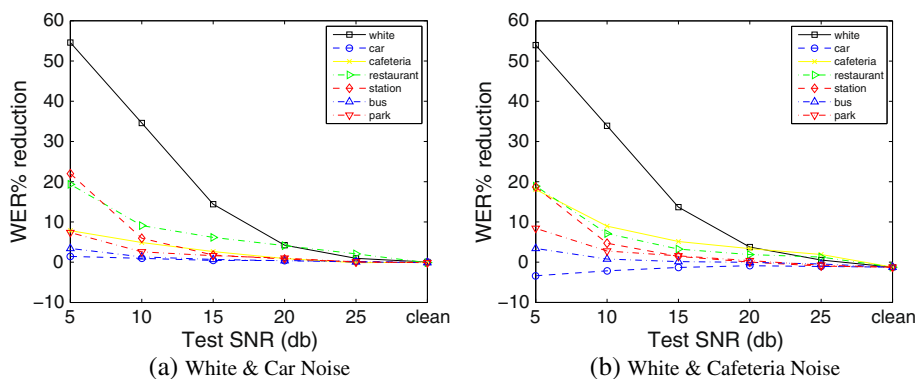
Figure 5 Performance of multiple noise injection. No clean speech is involved in training. (a) White and car noise. (b) White and cafeteria noise.
